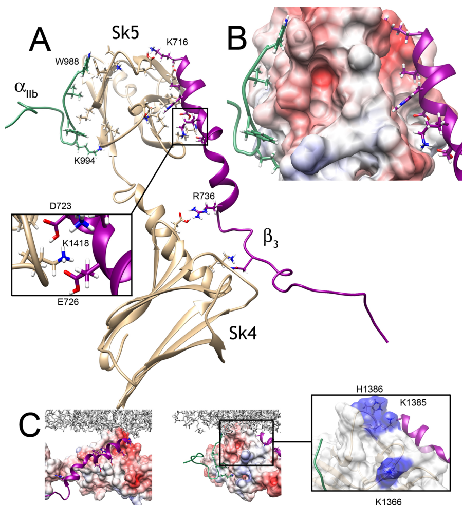
Figure 5. (A) Model of tertiary integrin/skelemin complex: Sk45 (tan) is shown bound to cytoplasmic tails of \alpha_{IIb} (green) and \beta_3 (purple) in ribbon presentation. Key residues are labeled. The inset shows a slightly rotated display of the hydrogen bonding network for a better view. (B) Zoomed view of the binding interface with Sk5 domain. The surface of Sk5 is colored based on its electrostatic potential. (C) The tertiary complex is arbitrarily placed with respect to the lipid bilayer represented by POPC and POPE mixture 27 shown in gray. Each side is shown to better visualize the binding pockets and potential orientation with the lipid bilayer. The inset depicts potentially positively charged residues of Sk5 domain (colored in blue) that may interact with the lipid bilayer.
