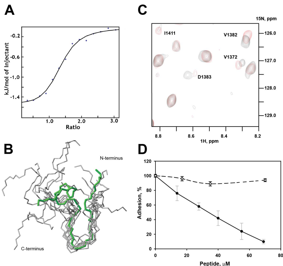
Figure 4. (A) ITC data for the Sk45 interaction with \alpha_{IIB} fitted with a single binding site model. (B) The NMR ensemble of \alpha_{IIB} cytoplasmic tail in the bound conformation as determined from trNOE data. The conformer used for docking is shown in green. (C) A region of the ^1\text{H} - ^{15}\text{N} HSQC spectra of Sk45 in absence (black) and presence of \beta_3 (red) at the protein/peptide ratio 1:3. Affected residues are labeled. (D) Effect of skelemin-derived peptide on \alpha_{IIB}\beta_3 -expressing CHO cell adhesion. Microtiter wells were coated with 2.5 \mu\text{g}/\text{mL} of fibrinogen and postcoated with 1% BSA. Calcein-labeled \alpha_{IIB}\beta_3 -expressing CHO cells were incubated with different concentration of THIVWYKDEREISVDEKHD (●) or control EREISAAAKHD (○) peptides for 20 min at 22 °C. After 30 min at 37 °C, nonadherent cells were removed, and adhesion was determined. Data points are expressed as a percentage of control adhesion (in the absence of peptides) and are the mean of three individual experiments performed with triplicate determinations in each experiment.
