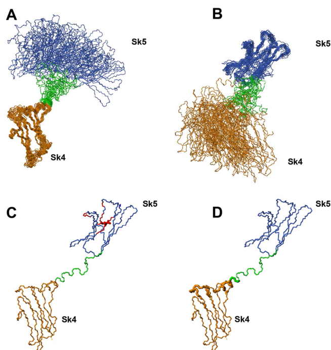
Figure 1. Sk45 NMR ensemble obtained through the calculation where RDC data for the two domains were used independently (A, B). Sk4 domain and N-terminal part of the linker is shown in orange, Sk5 domain—in blue, the unstructured part of the linker—in green. (A) The structures are superimposed over the domain 4 of the tandem Sk45 well-ordered residues 1227–1327. (B) The structures are superimposed over domain 5 of the tandem Sk45 well-ordered residues 1344–1380 and 1391–1427. Additional data used to confirm interdomains orientation (C–D). (C) The residues affected by the introduction of m-PROXYL spin label are in red. The spin modified residue is shown with the thicker bonds and side chain displayed. (D) The residues of Sk4 domain and the beginning of linker affected by the presence of the Sk5 domain are shown with thicker bonds. The affected residues were deduced from chemical shift perturbations in ^1\text{H} – ^{15}\text{N} HSQC spectra of Sk4 and Sk45 constructs.
