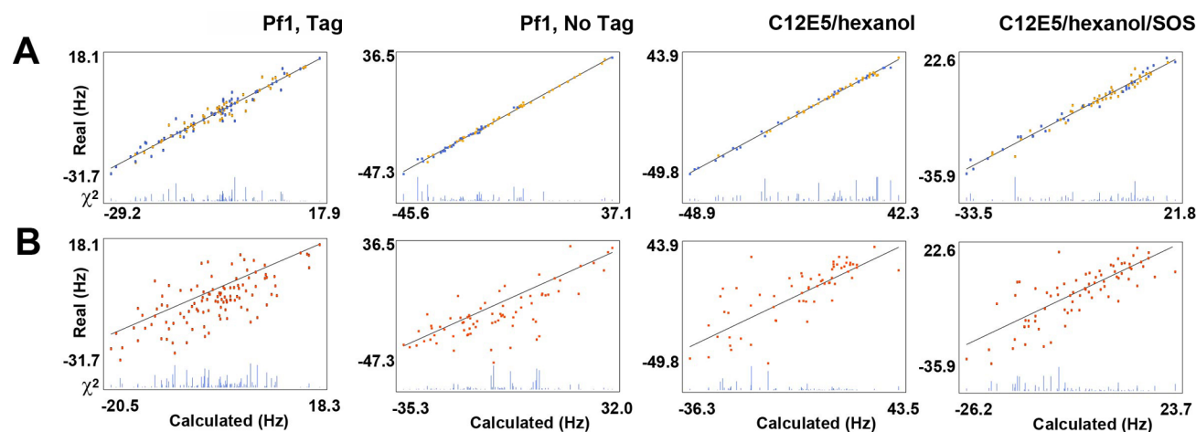
Figure 2. Quality of RDCs fits: the correlation fits of the experimental and back-calculated RDCs for the best structure from the NMR ensemble presented in Figure 1. (A) ^1\text{D}_{\text{HN}} RDCs data is split into two parts, one for each domain: data in orange corresponds to Sk4 domain and data in blue—to Sk5 domain. (B) The correlation fits of the experimental and back-calculated RDCs for the best structure from the NMR ensemble. These fits are obtained for ^1\text{D}_{\text{HN}} RDCs used as a single data set for the two domains. The four RDCs fits are (from left to right): Sk45 with His-tag in Pf1 anisotropic medium, Sk45 without tag in Pf1, C12E5/hexanol, or C12E5/hexanol/SOS media. The fits are obtained with MODULE. 26
