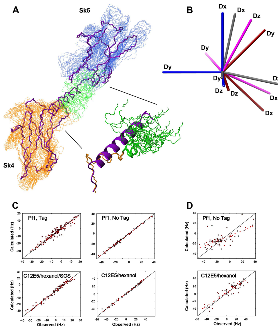
Figure 3. Overlay of Sk45 NMR ensemble with the X-ray structure of human homologue (PDB ID 3RBS) and the respective quality of RDCs fits. (A) The 20 lowest energy NMR structures with the two domains oriented by means of RDC data. The NMR ensemble and the X-ray structure (violet) are superimposed over residues 1227–1327 (domain Sk4) and 1344–1427 (domain Sk5). The linker region is magnified and is shown in ribbon presentation for X-ray structure. (B) The relative orientation of the alignment tensors for Sk45 with His-tag in Pf1 anisotropic medium (red), for Sk45 without tag in Pf1 (magenta), C12E5/hexanol (gray) or C12E5/hexanol/SOS (blue) anisotropic media. (C) The correlation fits of the experimental and back-calculated ^1\text{D}_{\text{HN}} RDCs for the best structure from the NMR ensemble of Sk45. (D) The correlation fits of the experimental and back-calculated ^1\text{D}_{\text{HN}} RDCs for the X-ray structure. The fits are obtained with Xplor-NIH tools.
